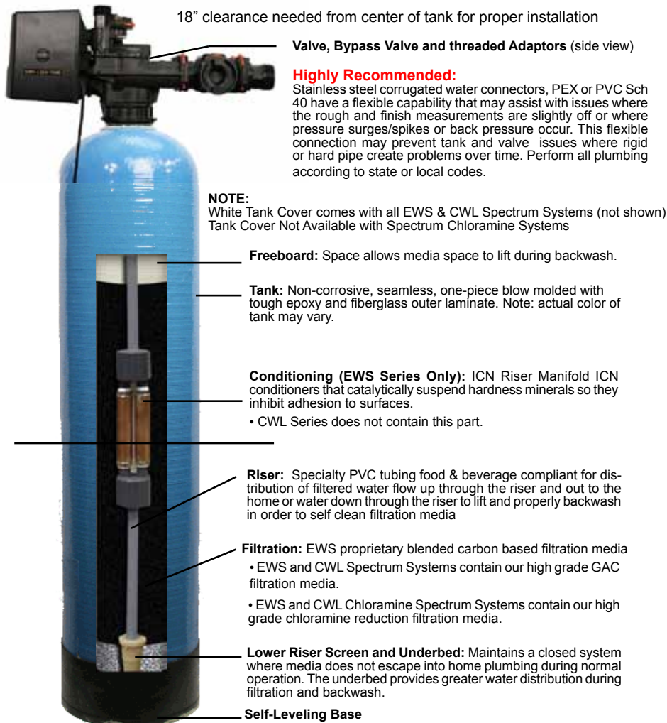
For Illustration Purposes Only: Cut-away of EWS Chloramine Spectrum System
